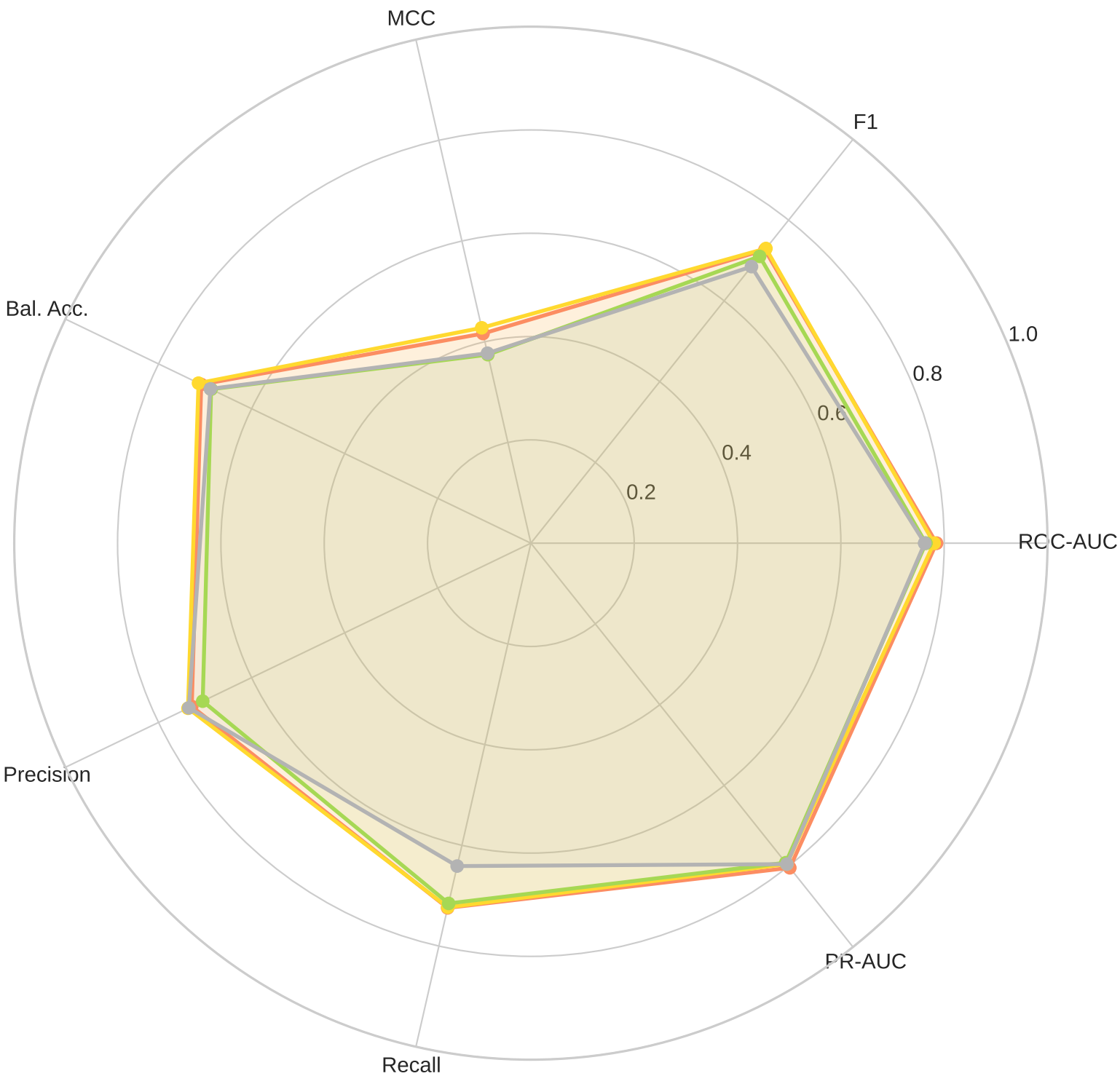
Multi-Metric Performance Comparison (Top 4 Models)
